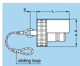
BFA Cap (for FHA and FWA plugs)
