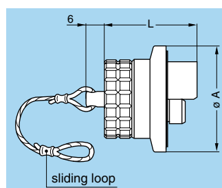
BFE Cap (for FHE and FWE plugs)
